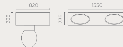
WC unit
