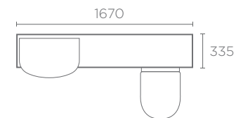
Basin unit
